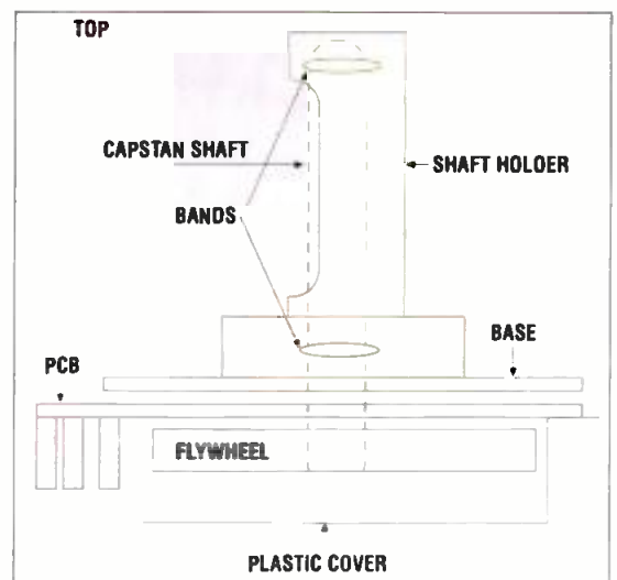
Figure 1: Sony BVW capstan and servo assembly.
