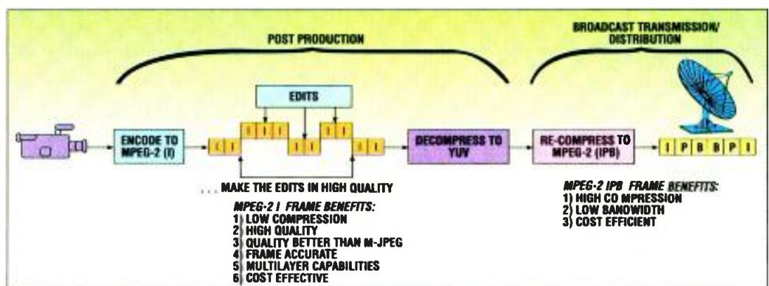
Figure 2. Typical signal path for broadcast distribution.
