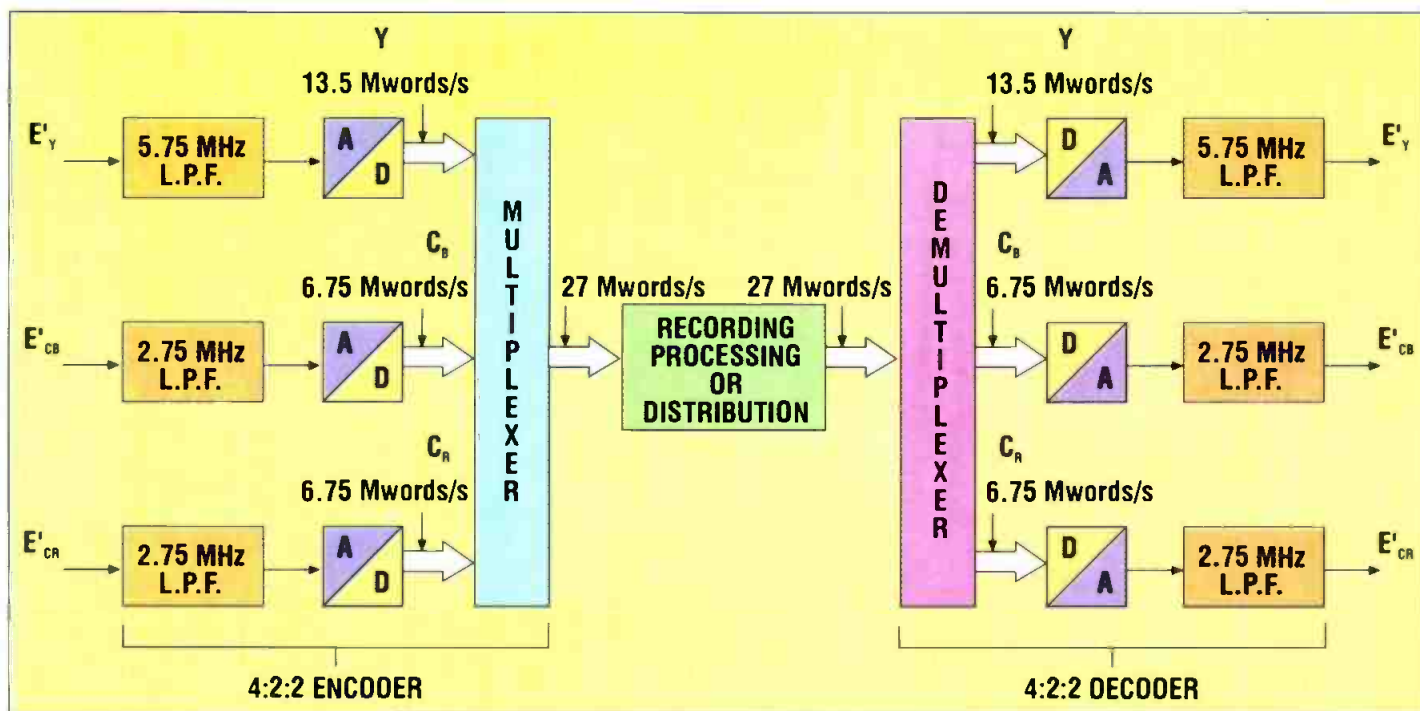
Figure 2. Simplified block diagram of 4:2:2 component digital system.
