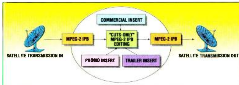
Figure 1. Typical signal path for satellite distribution.
